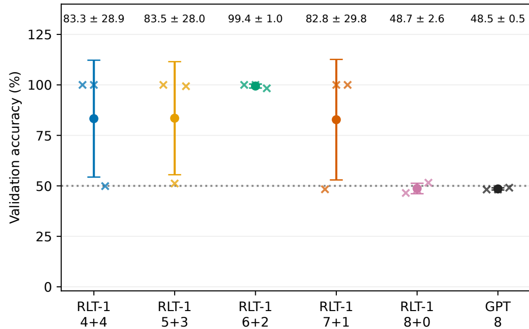
Step 500 · 256,000 training examples per seed
